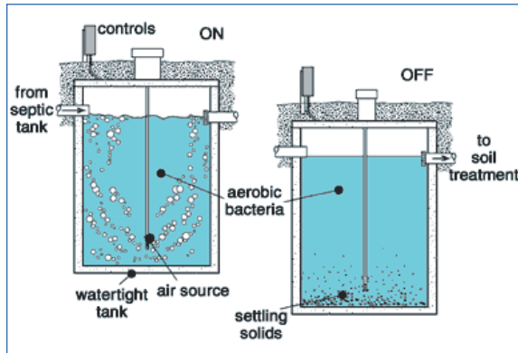
A sequencing batch reactor. Graphic: NSFC.
