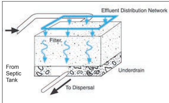
Single pass filter. Graphic: NSFC.
