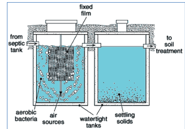
A fixed-film reactor. Graphic: NSFC.
